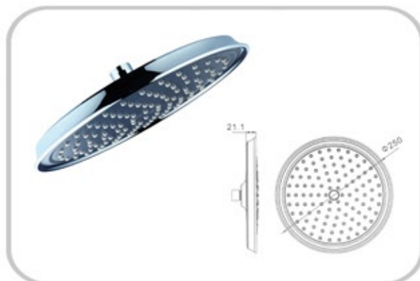
KSH-001-057 ABS shower head with nipple 10" (Ø 250 mm)
