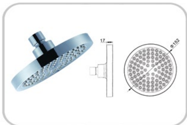
KSH-001-054 ABS shower head with nipple 6" (Ø152mm)
