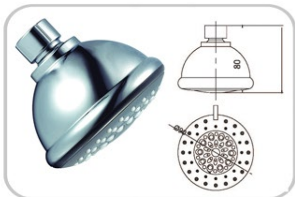
KSH-001-041C 1 setting shower head 4" (Ø 90 mm)
