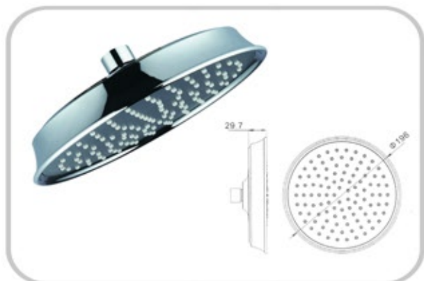
KSH-001-056 ABS shower head with nipple 8" (Ø 196 mm)
