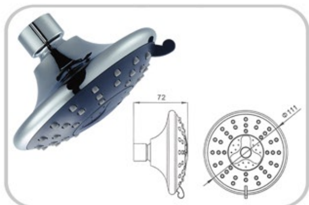
KSH-001-061 3 settings (spray / massage / mix) 4" (Ø 111 mm)
