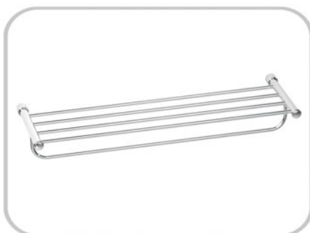
KHS-202 636 x 225 x 94.5 mm 25 x 8.9 x 3.7 inch
